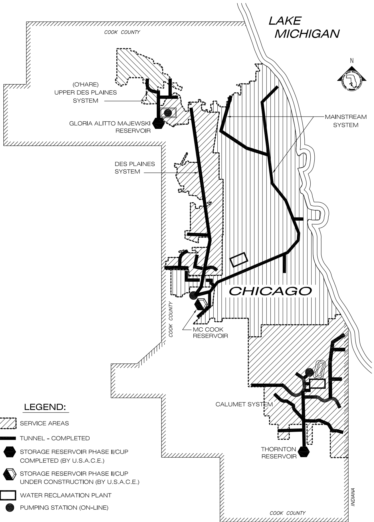
Tunnel and Reservoir Plan Project Status
