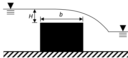
FIGURE 5.6 BROAD-CRESTED WEIR
