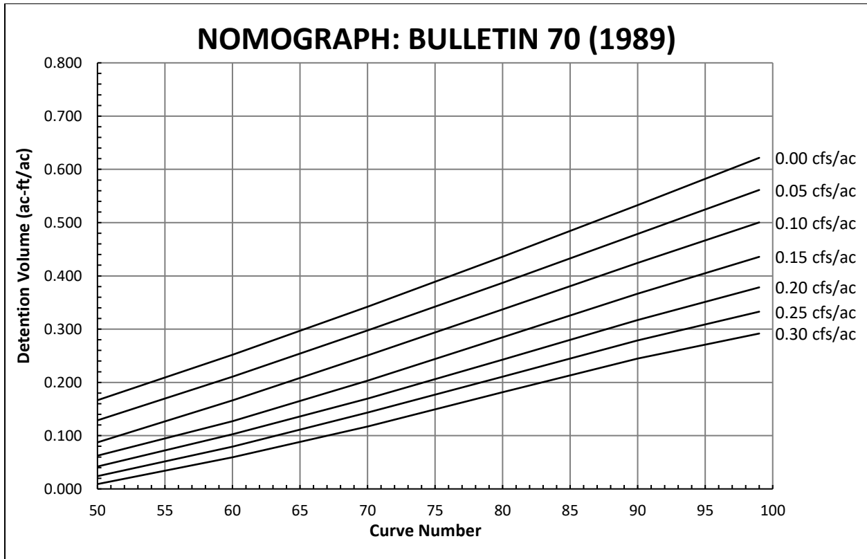
FIGURE 5.1 NOMOGRAPH FOR BULLETIN 70 (1989) RAINFALL DATA
