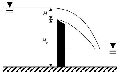
FIGURE 5.3 SHARP-CRESTED WEIR (FREE-FLOW CONDITION)
