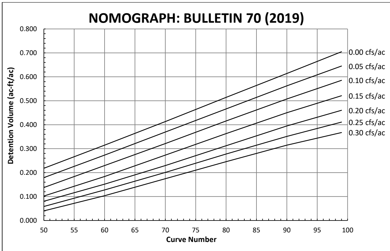
FIGURE 5.2: NOMOGRAPH FOR BULLETIN 70 (2019) RAINFALL DATA
