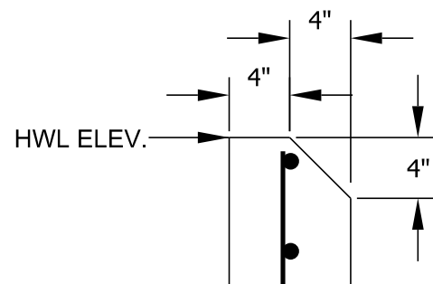
BAFFLE WALL DETAIL
