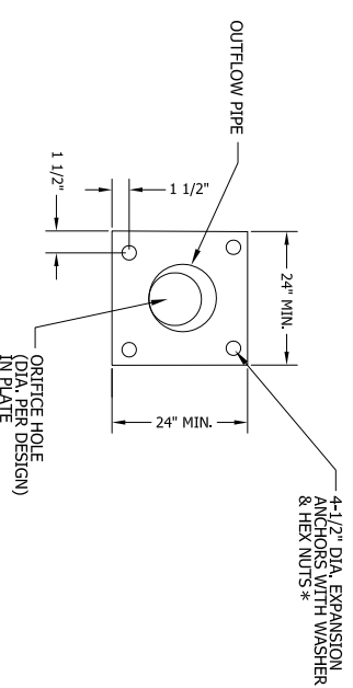
PLATE RESTRICTOR DETAIL: ELEVATION
