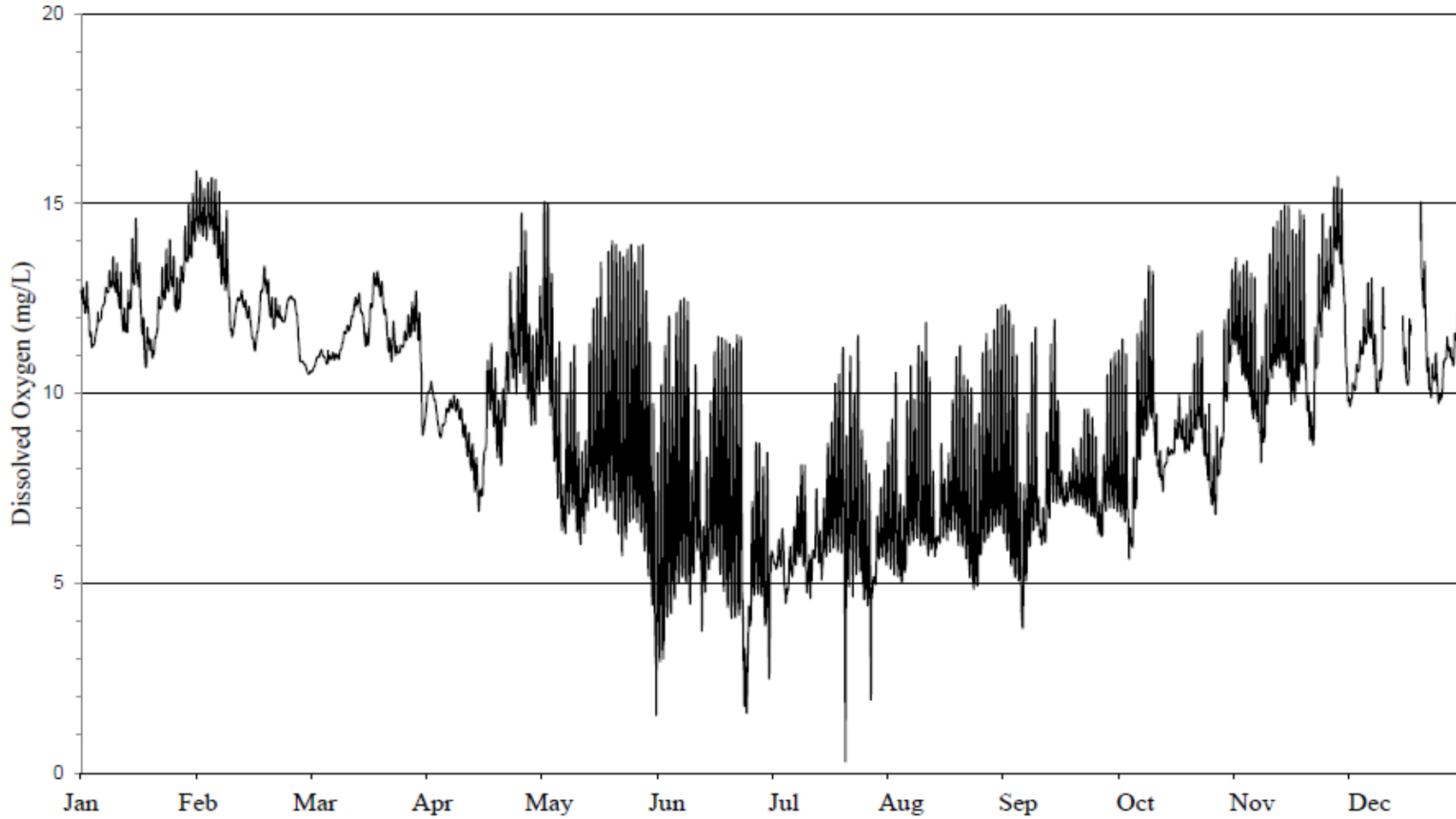
FIGURE 20: DISSOLVED OXYGEN CONCENTRATION MEASURED HOURLY AT OGDEN AVENUE ON THE DES PLAINES RIVER FROM JANUARY 1, 2023, THROUGH DECEMBER 31, 2023
