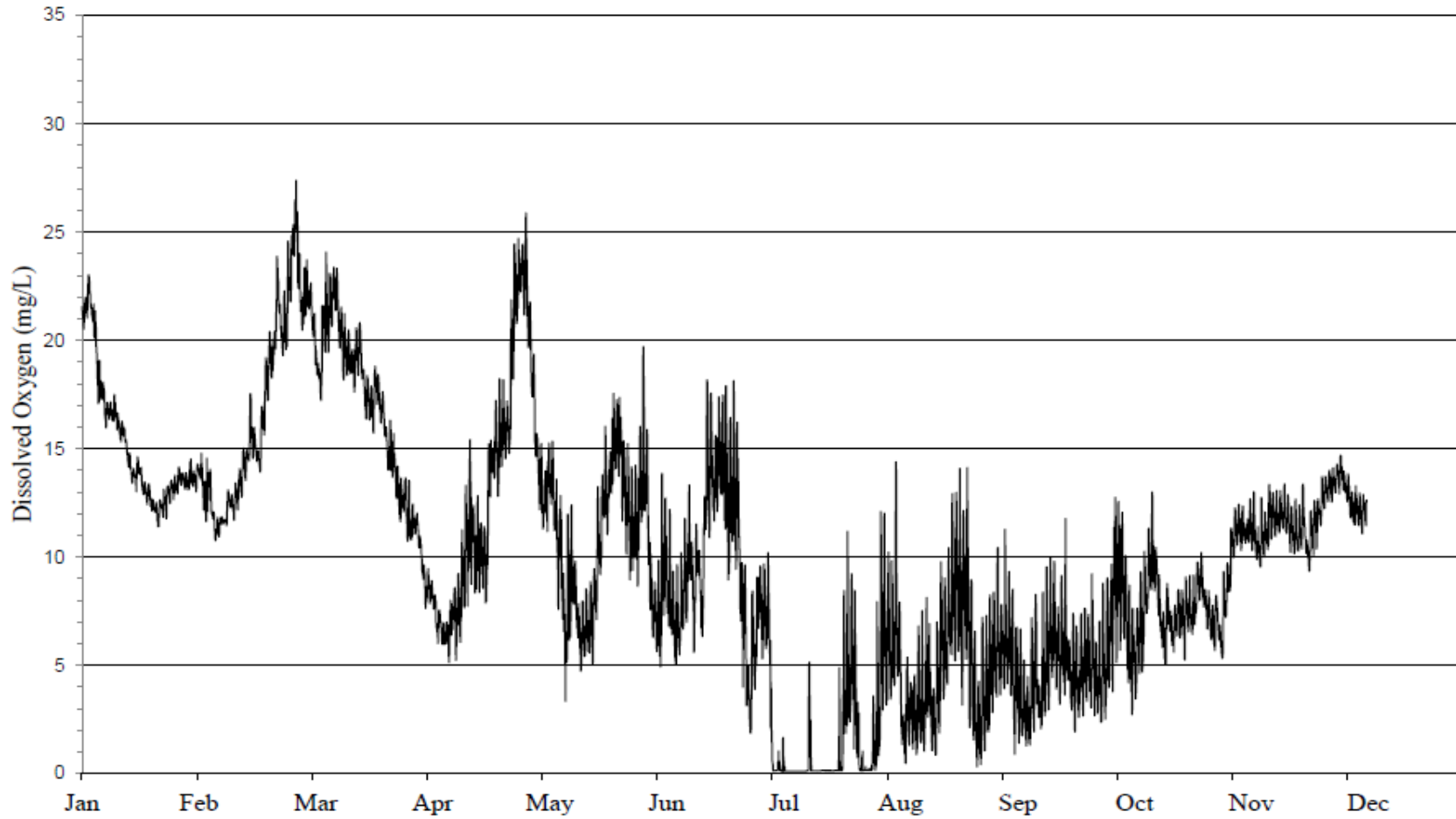
FIGURE 8: DISSOLVED OXYGEN CONCENTRATION MEASURED HOURLY AT 36 TH STREET ON BUBBLY CREEK FROM JANUARY 1, 2023, THROUGH DECEMBER 31, 2023
